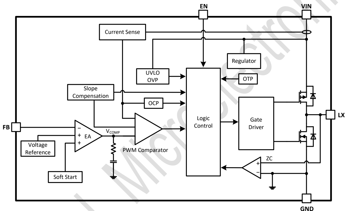
Figure 2. TMI3408 Block Diagram
