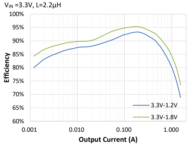
Efficiency at V_{IN}=3.3V
